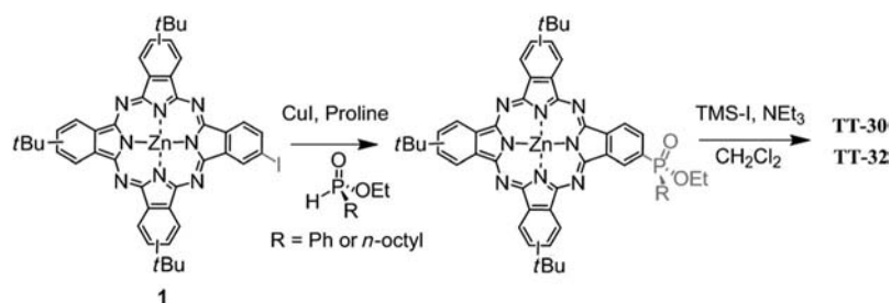
Scheme 2. Synthesis of TT-30 and TT-32 dyes. TMS = trimethylsilyl.
